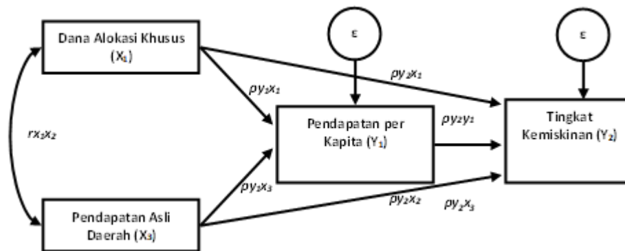
Figure 1 Path Analysis
